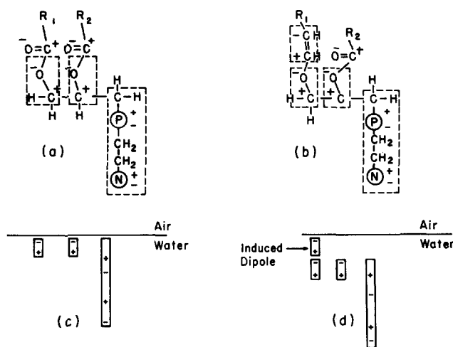
FIG. 3. Structure of lecithin (a) and phosphatidyl choline (b); the corresponding dipole components, (c) and (d). R 1 and R 2 represent the hydrocarbon chains. P and N represent the phosphate and the trimethylammonium groups. + and - are to be understood as meaning partial charges, \delta^+ and \delta^- respectively.
