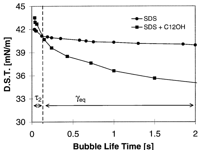
FIG. 6. Dynamic surface tension ( \gamma_D ) of SDS and SDS/C 12 OH mixtures at 25°C (15 mM SDS, 5 mol% C 12 OH).
