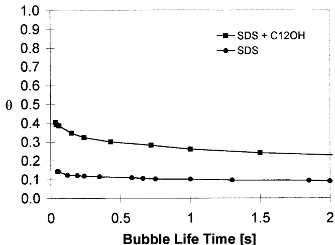
FIG. 7. Dimensionless dynamic surface tension ( \theta ) of SDS and SDS/ C_{12}OH mixtures at 25°C (15 mM SDS, 5 mol% C_{12}OH ).
