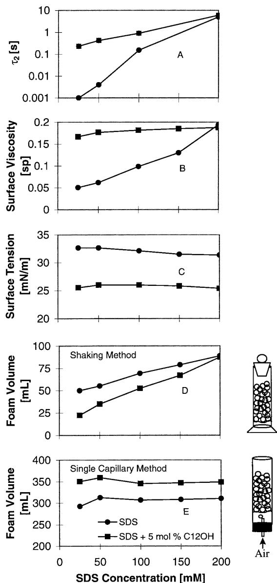
FIG. 5. The effect of 5 mol% C 12 OH on foaming properties of SDS solutions.
