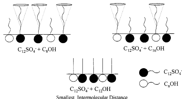
FIG. 3. Schematic diagram showing the effect of chain length compatibility on molecular packing at the interface.
