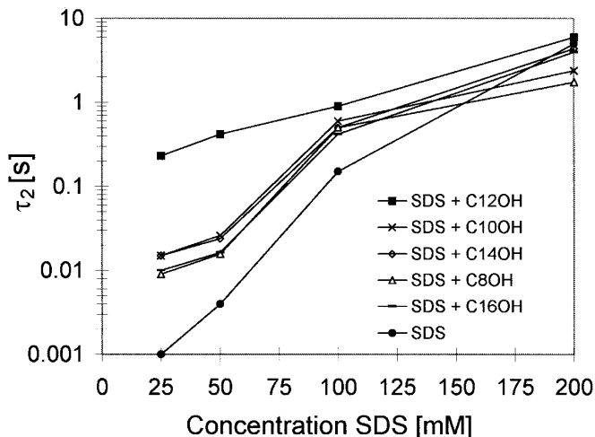
FIG. 1. The effect of 5 mol% C_n OH on the micellar relaxation time ( \tau_2 ) in SDS solutions at 25°C.
