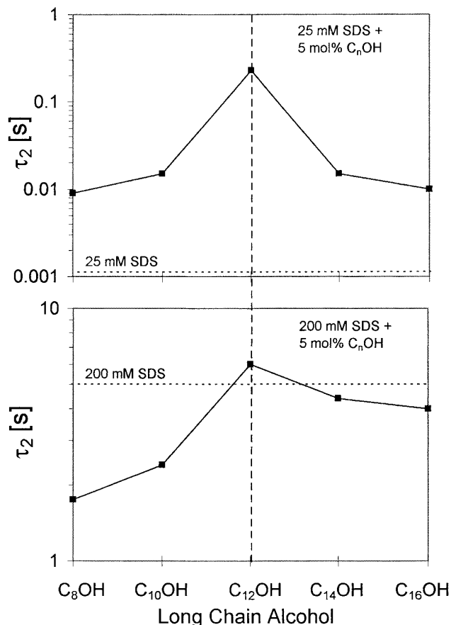
FIG. 2. The effect of 5 mol% C_n OH on the micellar relaxation time ( \tau_2 ) of 25 and 200 mM SDS solutions at 25°C.
